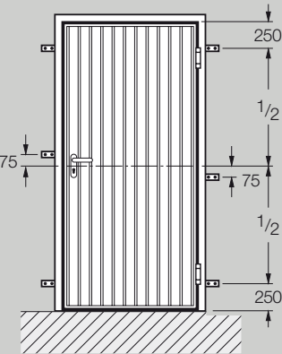
Position of anchors
